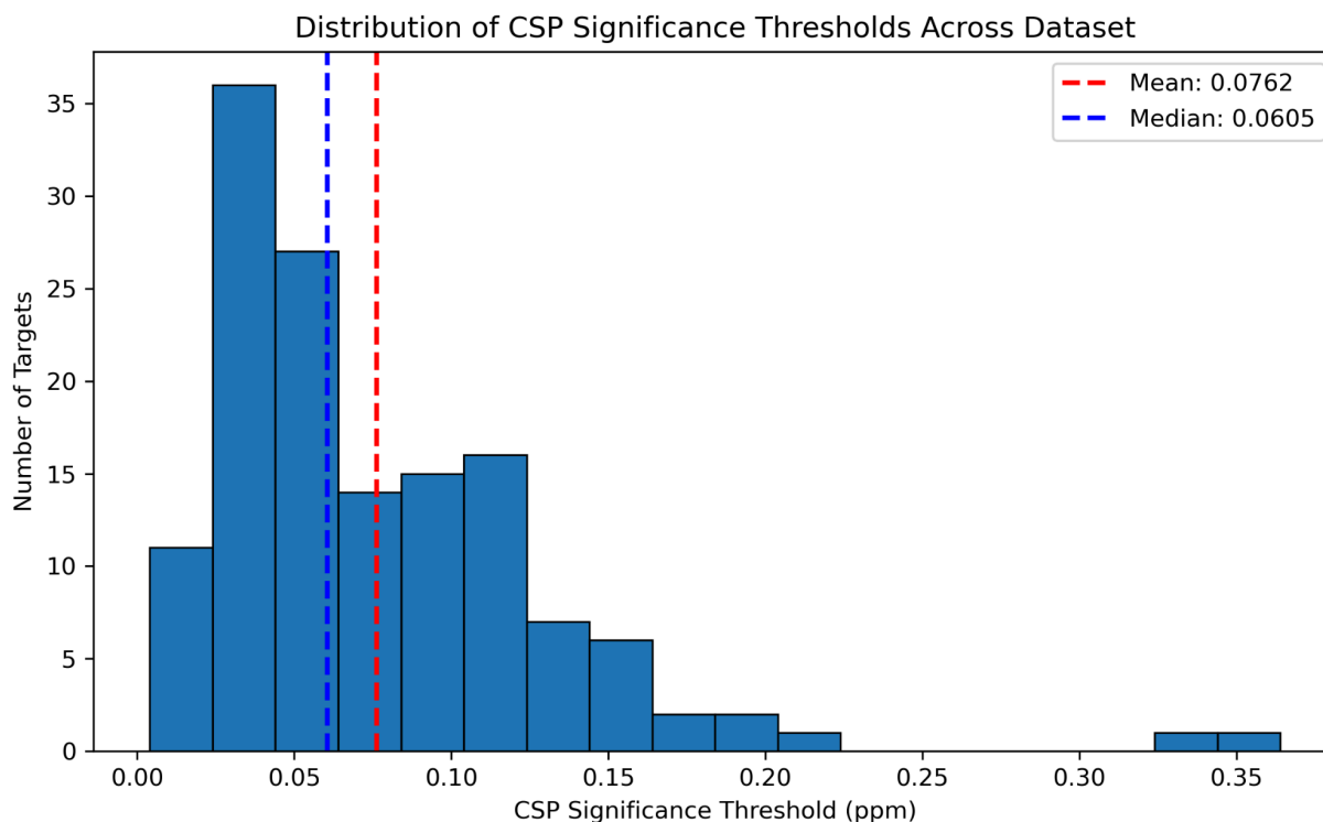
SI Fig. S17. CSP significance threshold Histogram. This histogram summarizes the thresholds for determining whether a CSP for a given receptor is significant. For a small number of targets, the calculated significance threshold is significantly higher than one would expect, we attribute this to differences in experimental conditions between the apo and holo NMR experiments which aberrantly perturbs all observed shifts. We prune from the CSPdb any targets with a calculated significance threshold > 0.6 ppm. This includes the following targets: 2LMC, 1OO9, 2L12, 2L00, 2N01, 2MP0, 8VOI, 8U2Y, 6OSW.
