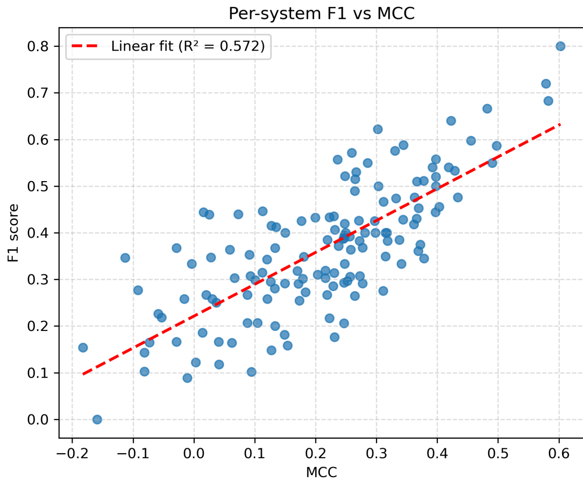
SI Fig. S18. F1 vs MCC score comparison across CSP DB targets. This plot shows the correlation between calculated F1 and MCC metrics. MCC is a more reliable metric for larger systems with many True Negatives (small CSPs outside of the binding site) (7).
