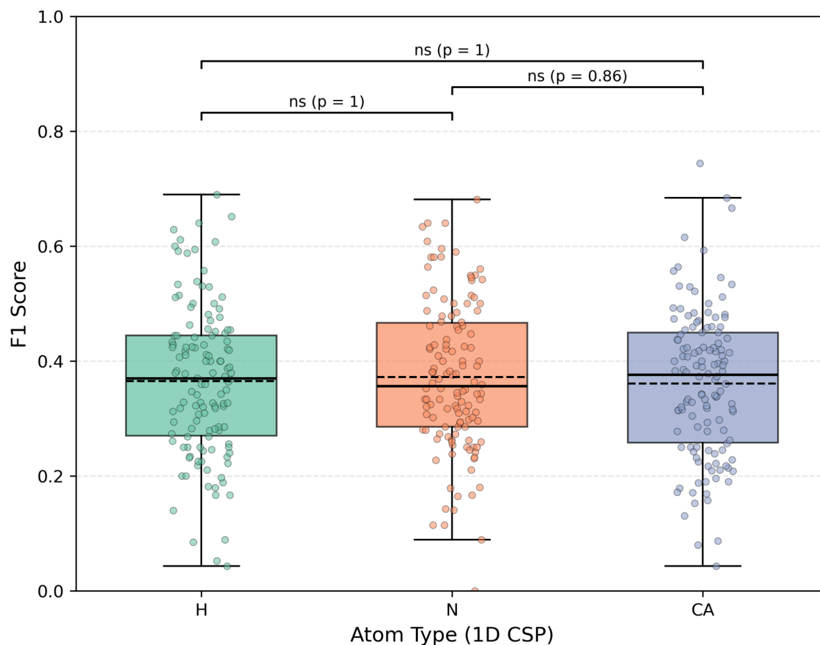
SI Fig. S14. F1 Scores for 1D CSPs. This plot shows there are no statistical differences between distributions of calculated F1 scores from 1D CSPs H/N/CA atom types. CSPs are calculated as root-squared differences after applying an ideal holo offset for a 3D H/N/CA offset grid (see Methods for details). Statistical analysis is performed using paired Wilcoxon tests with Holm correction.
