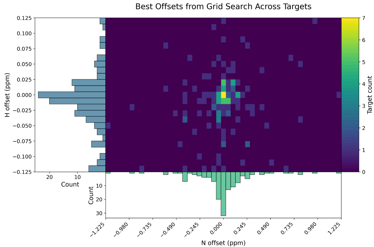
SI Fig. S16. Ideal offsets across the whole dataset for N/H. This heatmap shows the offsets used to align the apo/holo HSQC plots. The majority of targets require small adjustments within 0.025 ppm on the Hydrogen axis and 0.245 ppm on the Nitrogen axis.
